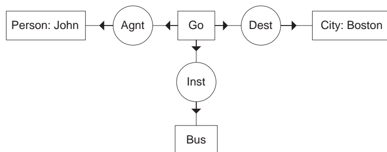
Figure 2.8: Conceptual Graph for “John goes to Boston by bus”
