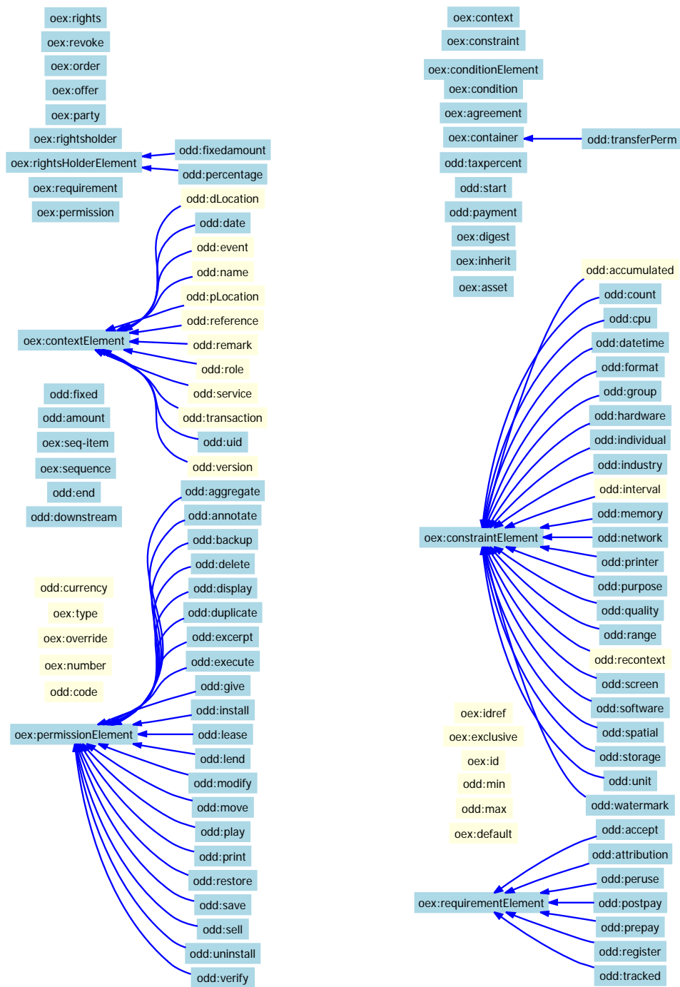
Figure 11.2: ODRL XML elements and attributes formalised as OWL properties hierarchies
